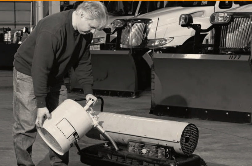
JUS11202Y Polypropylene Funnel for use with Type I Safety Can
