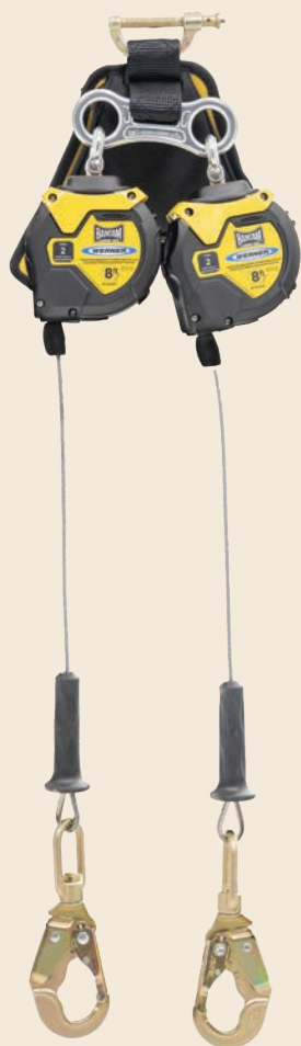
WCR413008LE 8 ft. Bantam Twin Leg Self-Retracting Lifeline, Leading Edge Capability $699 Meets ANSI z359.14-2021, Class 2; OSHA Standards
